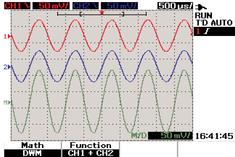
Figure 3 The U1600A series comes equipped with DWM features, allowing you to perform spectrum analysis and evaluate signal addition and subtraction from multiple channels.
