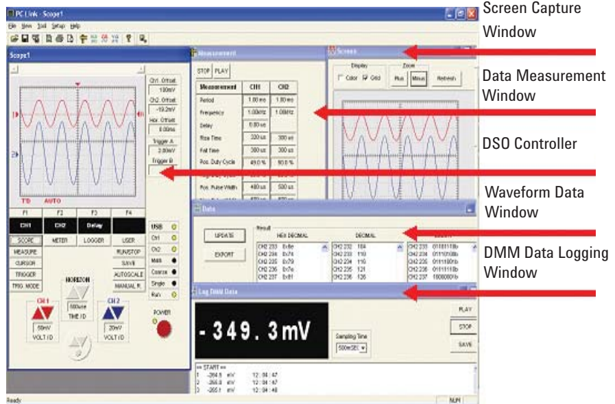
Figure 4 The U1600A series comes with a PC Link application software that caters for data gathering, storage and documentation needs via USB full speed remote control from PC.
